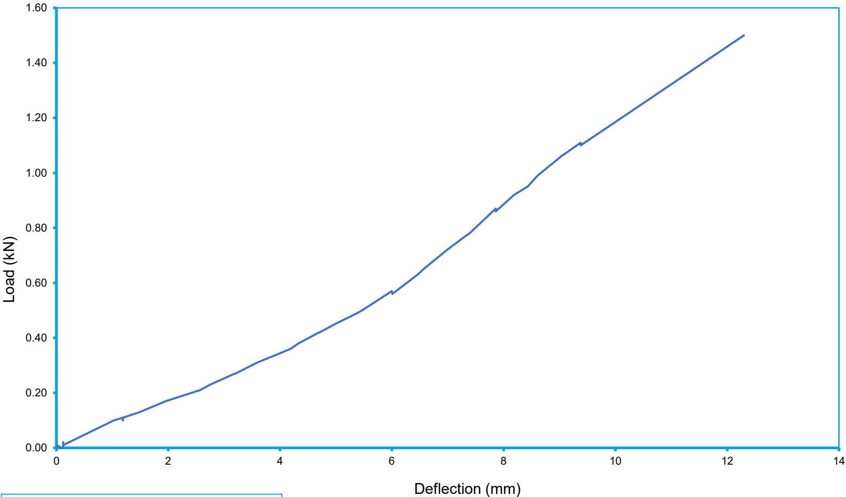
Chart 2 - Load Deflection Curve for Point Load Testing of SWR Round Modular 42.4 mm Base Mounted Balustrade Systems
