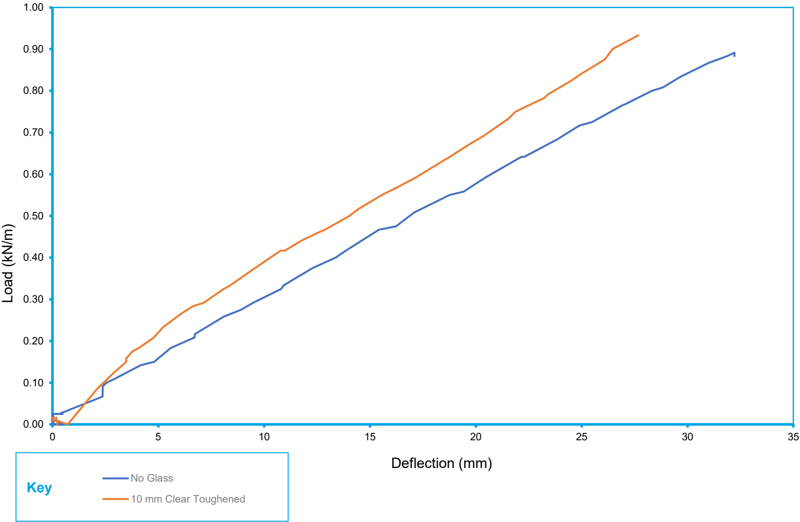
Chart 1 - Load Deflection Curve for Uniformly Distributed Line Load Testing of SWR Round Modular 42.4 mm Base Mounted Balustrade Systems
